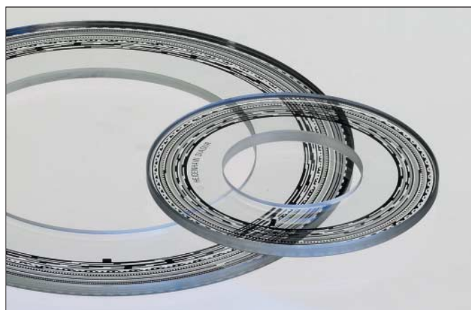
Circular graduations of absolute angle encoders
