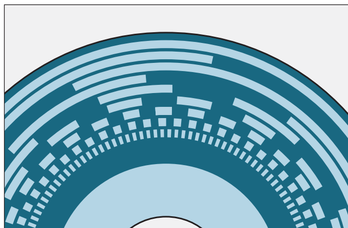
Schematic representation of a circular scale with absolute grating
