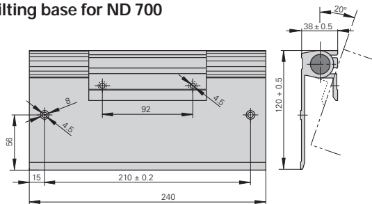
Tilting base for ND 700
