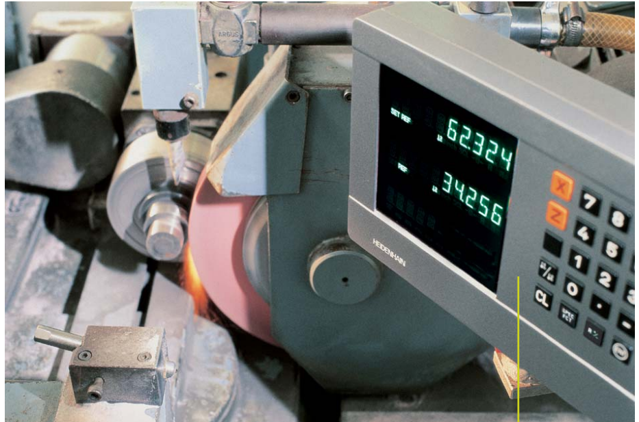
Circular grinding p. 12 ND 730 display unit Linear encoders on X and Z: LS 406 C Display step: 1 \mu\text{m}
