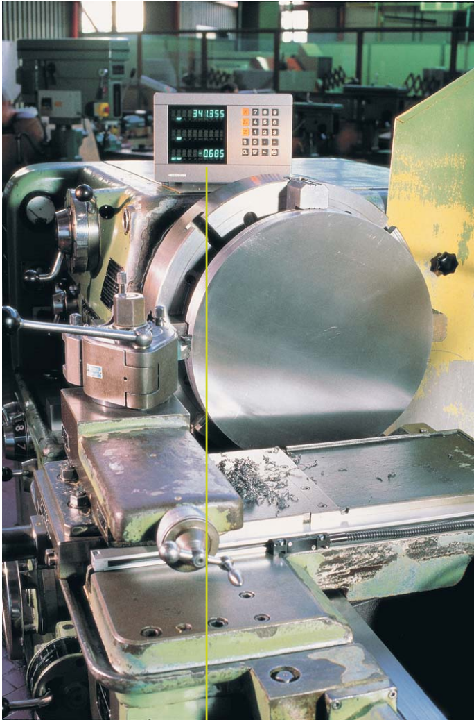
Turning p. 12 ND 770 display unit (sum display Z and Z 0 ) Linear encoders on X and Z 0 : LS 303 C On Z: LS 603 C Display step: 5 µm
