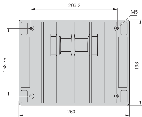
Tilting base for ND 700
