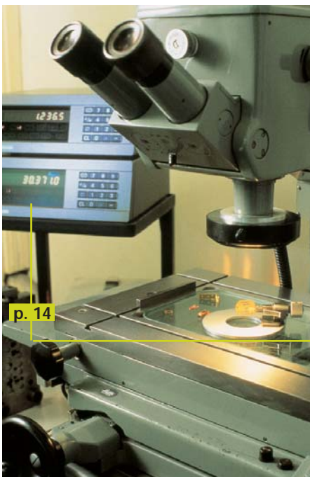
Measuring and inspection p. 14 ND 281 B display unit Linear encoders on X and Y: LS 406 C Display step: 0.5 µm
