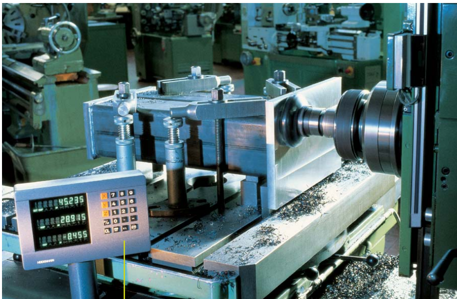
Milling p. 12 ND 760 display unit Linear encoders on X and Y: LS 603 C , On Z: LS 303 C Display step: 5 \mu\text{m}
