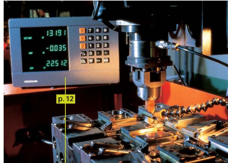
Eroding p. 12 ND 750 display unit Linear encoders on X and Y: LS 106 C On Z: LS 406 C Display step: 1 µm
